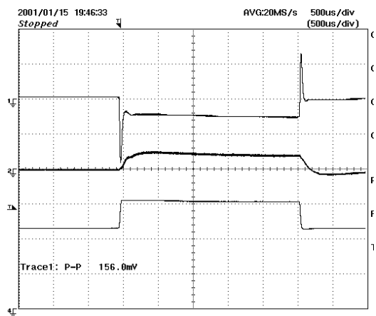
Figure 22 - 5 V and 3.3 V Transient Response. 75-100-75% Load Step 5 V output. Upper: 5 V, 100 mV / div. Middle: 3.3 V, 100 mV / div. Bottom: 5 V output current, 1 A / div. 500 \mu s / div.
